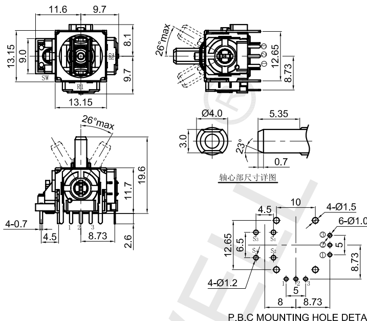
P.B.C MOUNTING HOLE DETAIL
